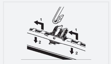
ADAPTER H24
