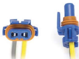
Cod. 40788 Imballo Packaging 1 Pcs. Tipo Lampada / Bulb Type HB3-9005 Base P20d
