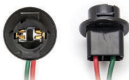
Cod. 40748 Imballo Packaging 1 Pcs. Tipo Lampada / Bulb Type T10 Base W2,1x9,5d
