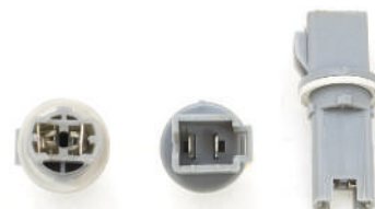
Cod. 40765 Imballo Packaging 1 Pcs. Tipo Lampada / Bulb Type T10 Base W2,1x9,5d
