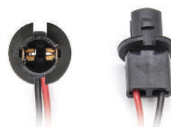
Cod. 40734 Imballo Packaging 1 Pcs. Tipo Lampada / Bulb Type T10 Base W2,1x9,5d
