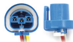
Cod. 40791 Imballo Packaging 1 Pcs. Tipo Lampada / Bulb Type HB5-9007 Base PX29t
