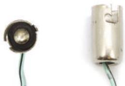
Cod. 40792 Imballo Packaging 1 Pcs. Tipo Lampada / Bulb Type T8,5 Base BA9S
