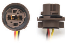
Cod. 40773 Imballo Packaging 1 Pcs. Tipo Lampada / Bulb Type T20 Base W3X16q
