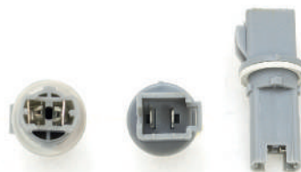
Cod. 40765 Imballo Packaging 1 Pcs. Tipo Lampada / Bulb Type T10 Base W2,1x9,5d
