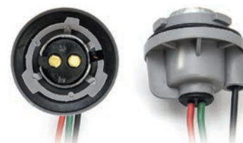
Cod. 40721 Imballo Packaging 1 Pcs. Tipo Lampada / Bulb Type PY21/5W Base BAY15D
