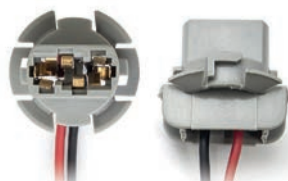
Cod. 40780 Imballo Packaging 1 Pcs. Tipo Lampada / Bulb Type W21W - 7440 Base W3X16d
