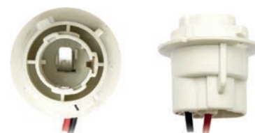
Cod. 40732 Imballo Packaging 1 Pcs. Tipo Lampada / Bulb Type P21W Base BA15S
