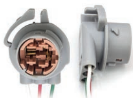
Cod. 40779 Imballo Packaging 1 Pcs. Tipo Lampada / Bulb Type P27/7W (3157) Base W2,5X16q
