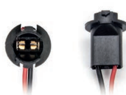
Cod. 40746 Imballo Packaging 1 Pcs. Tipo Lampada / Bulb Type T10 Base W2,1x9,5d
