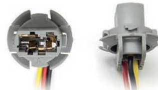
Cod. 40781 Imballo Packaging 1 Pcs. Tipo Lampada / Bulb Type W21/5W - 7443 Base W3X16q
