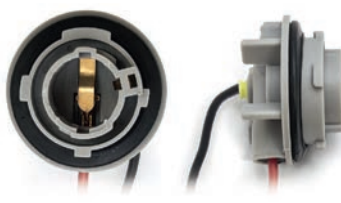
Cod. 40727 Imballo Packaging 1 Pcs. Tipo Lampada / Bulb Type P21W Base BA15S
